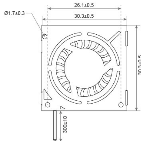
DIMENSIONS DRAWING UNIT : mm
