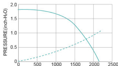
P&Q Curve At Rated Voltage
