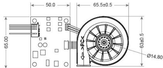
DIMENSIONS DRAWING UNIT : mm
