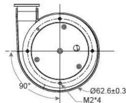
DIMENSIONS DRAWING UNIT : mm
