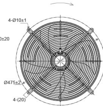
DIMENSIONS DRAWING UNIT : mm
