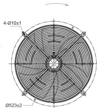
DIMENSIONS DRAWING UNIT : mm
