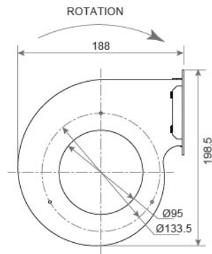
DIMENSIONS DRAWING UNIT : mm
