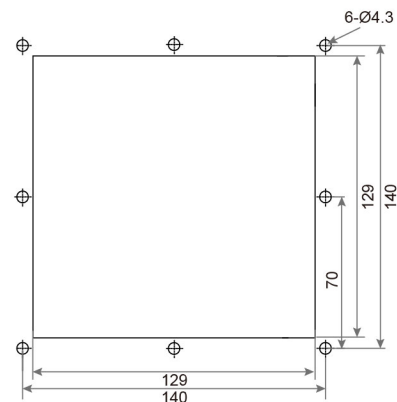
PANEL OPENING SIZE
