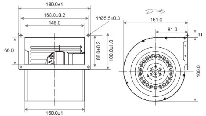
DIMENSIONS DRAWING UNIT : mm
