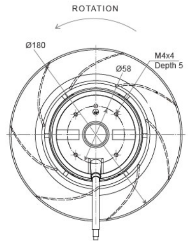
DIMENSIONS DRAWING UNIT : mm
