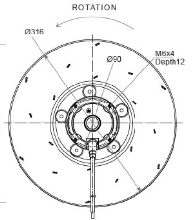
DIMENSIONS DRAWING UNIT : mm
