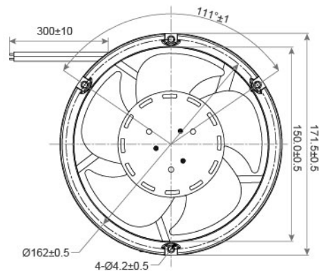
DIMENSIONS DRAWING UNIT : mm
