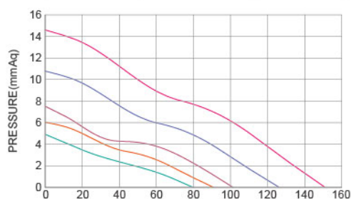
P&Q Curve At Rated Voltage
