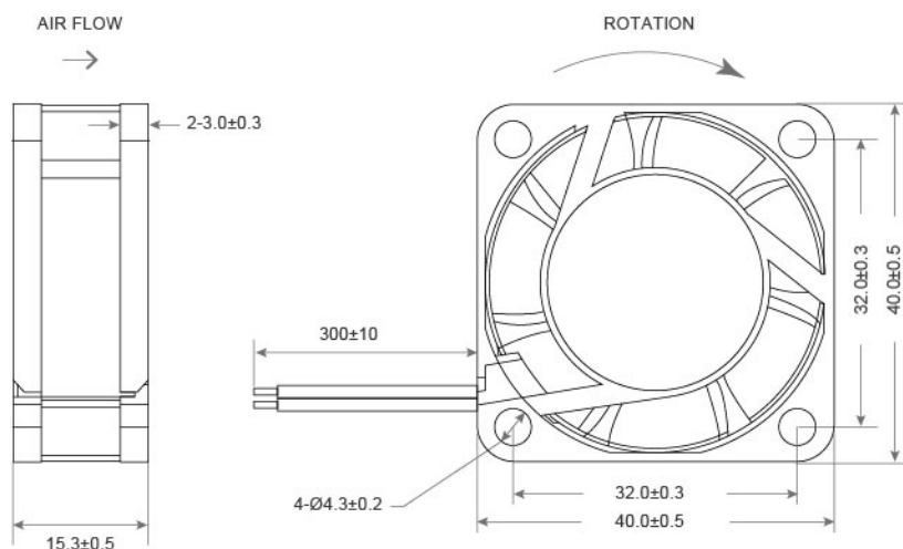
DIMENSIONS DRAWING UNIT : mm
