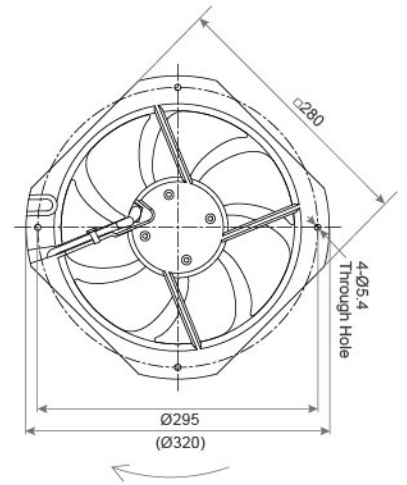
DIMENSIONS DRAWING UNIT : mm
