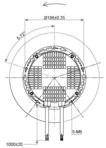
DIMENSIONS DRAWING UNIT : mm
